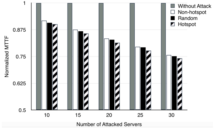
Fig. 13: Thermal attacks on a rack significantly reduces the server MTTF. A hotspot attack is shown to be more effective because of its consideration of air recirculation.
